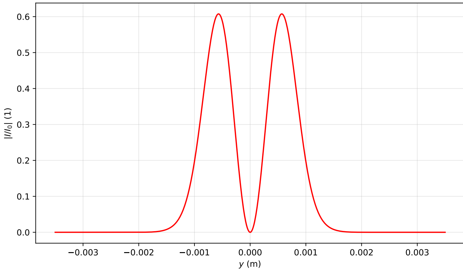
Intensity profile I(x=0, y, z=1.035)/I_0 , P_{in}=0.5P_{cr} , artificial time
